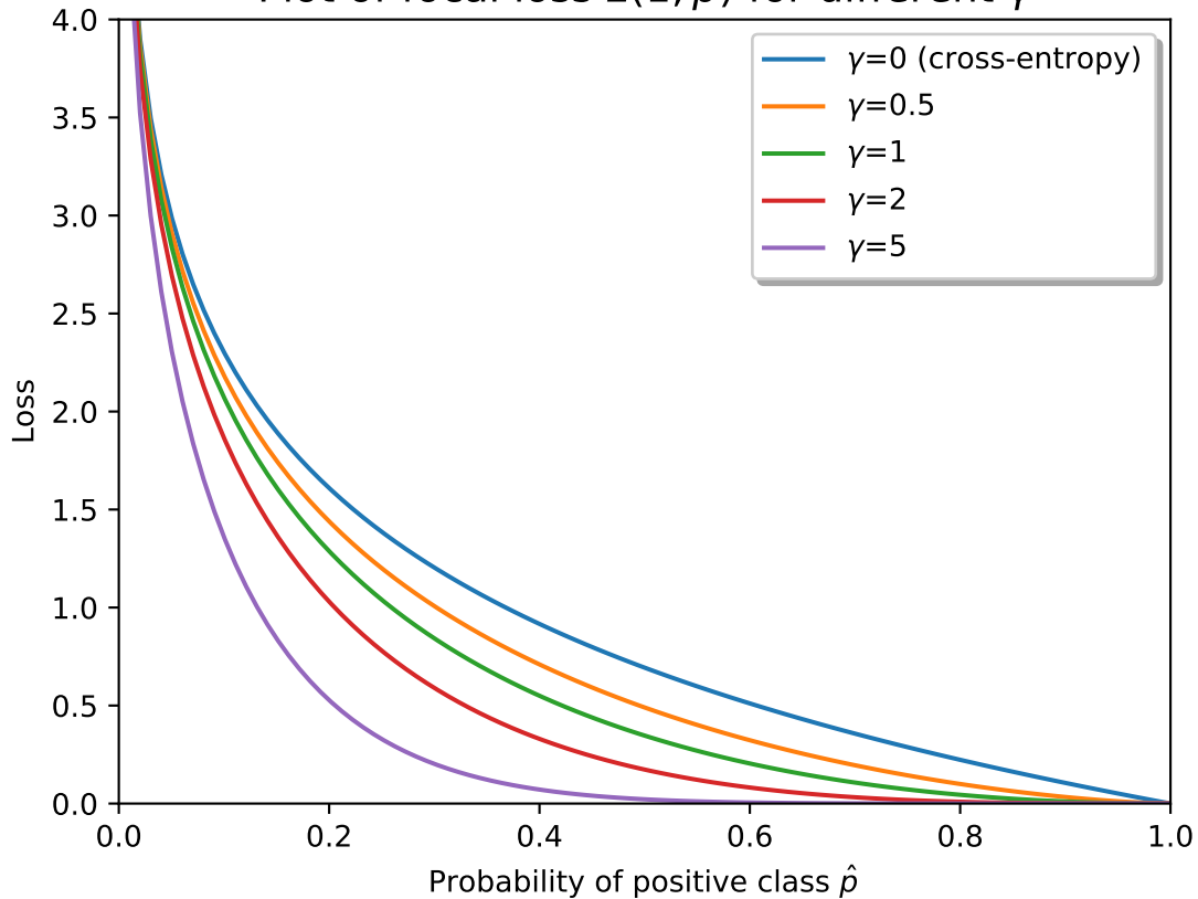
Plot of focal loss L(1, \hat{p}) for different \gamma
